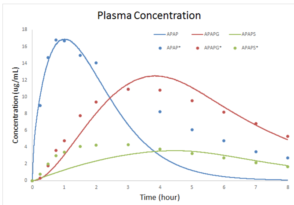
Adsorption, Distribution, Metabolism and Excretion (ADME) data (points), along with the reference model output (lines), for an oral 1g dose of APAP in humans.
